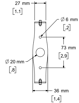
Rear View BRACKET ONLY
